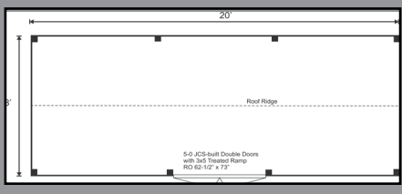
Option A Floor Plan
